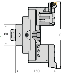
Complete tool
