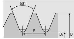
MJ Coarse pitch thread in accordance with DIN ISO 5855
