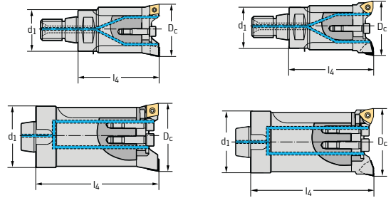
Complete tool
