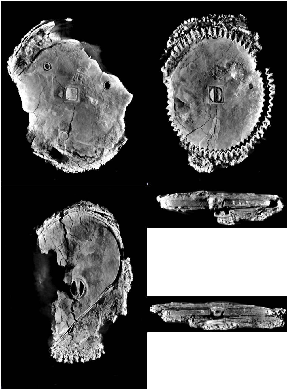
Fig. 32 X-ray CT of Fragment D. ©2005 Antikythera Mechanism Research Project. All rights reserved.
