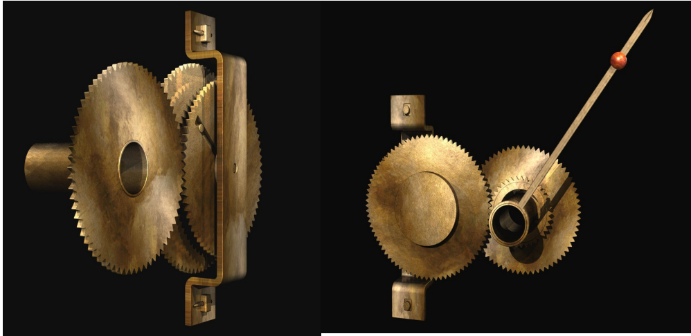
Fig. 35 Computer Reconstruction of Mars Mechanism. ©2011 Tony Freeth, Images First Ltd. All rights reserved.
