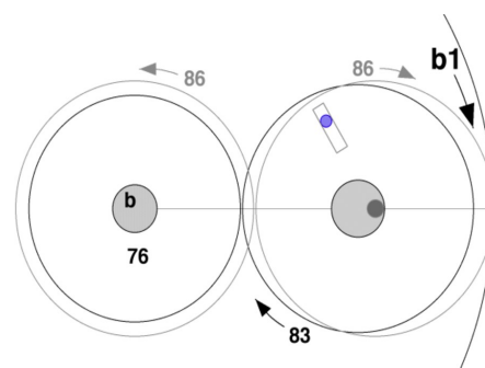
Jupiter—based on 83 synodic cycles in 76 years.
