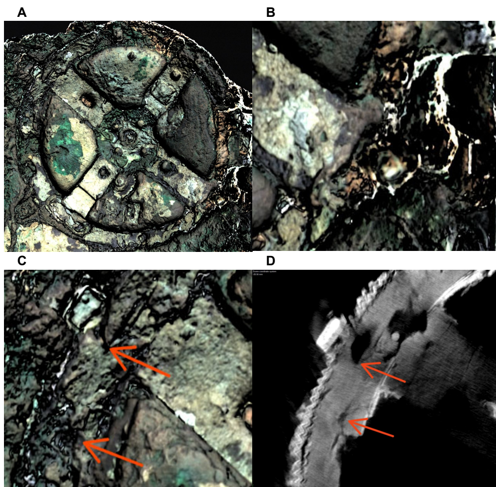
Fig. 22 Short pillar attachments on the Main Drive Wheel. ©2005 Antikythera Mechanism Research Project. All rights reserved.
