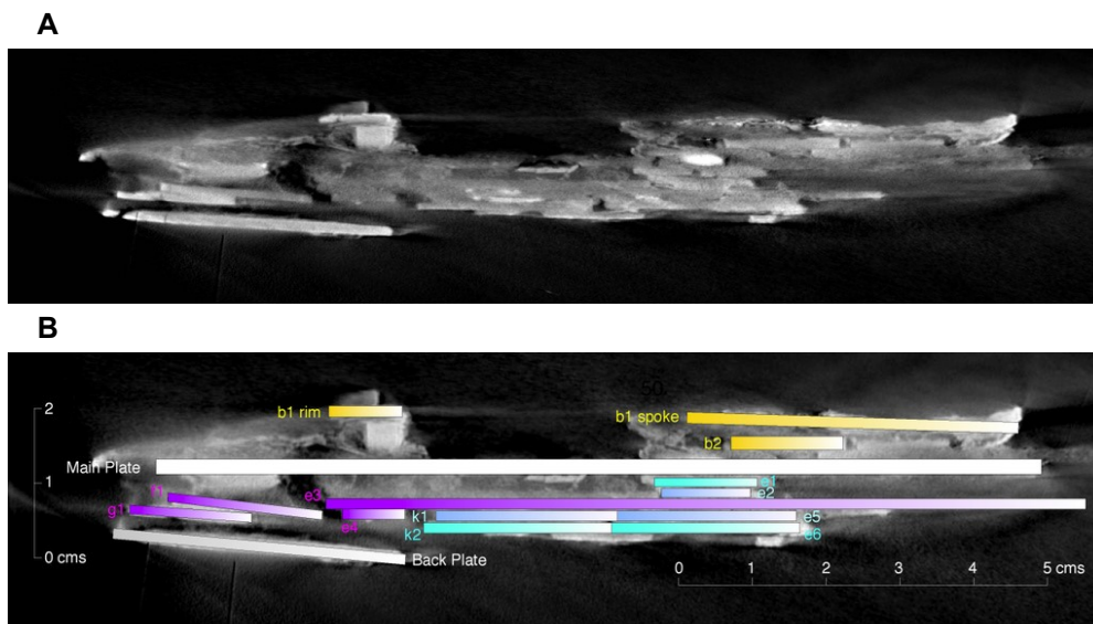
Fig. 7 X-ray CT showing cross-section of gearing in Fragment A. ©2005 Antikythera Mechanism Research Project. All rights reserved.
