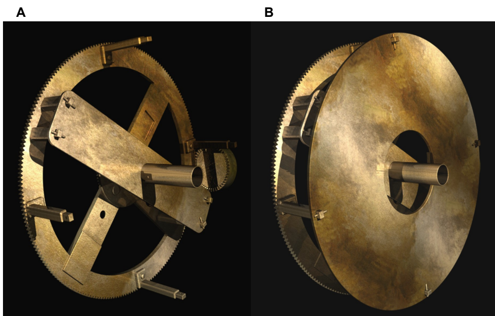
Fig. 29 Computer reconstruction of b1 with plates carried by the pillars. ©2011 Tony Freeth, Images First Ltd. All rights reserved.
