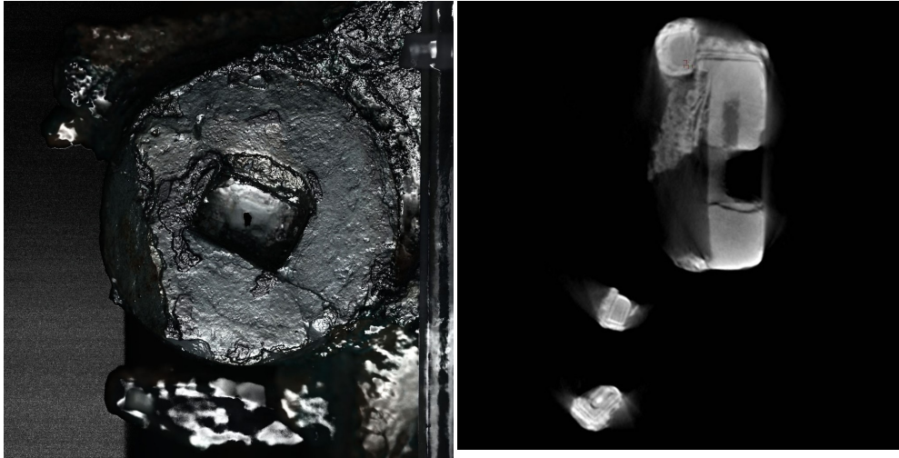
Fig. 17 Fragment A-1, showing the support pillars attached to b1. ©2005 Antikythera Mechanism Research Project. All rights reserved.
