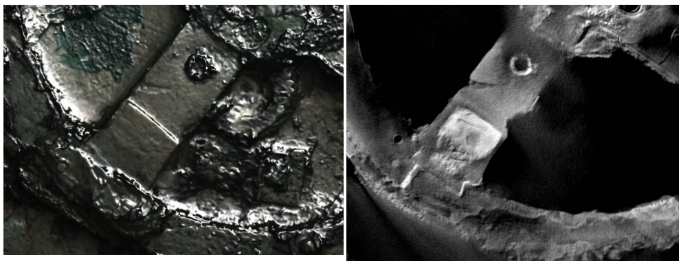
Fig. 15 Flattened area on the spoke in the 7 o'clock position. ©2005 Antikythera Mechanism Research Project. All rights reserved.
