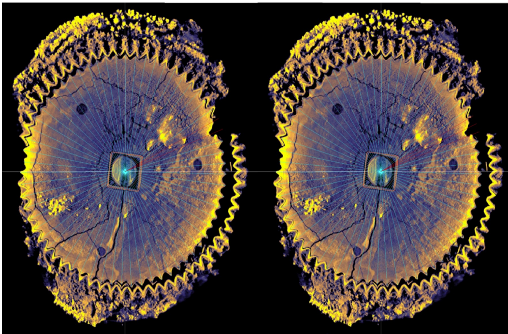
Fig. 33 X-ray CT section of gear in Fragment D. ©2005 Antikythera Mechanism Research Project. All rights reserved.
