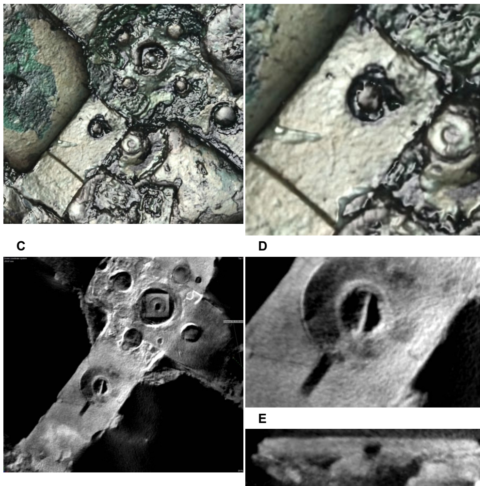
Fig. 14 Apparent bearing in the 7 o'clock position. ©2005 Antikythera Mechanism Research Project. All rights reserved.
