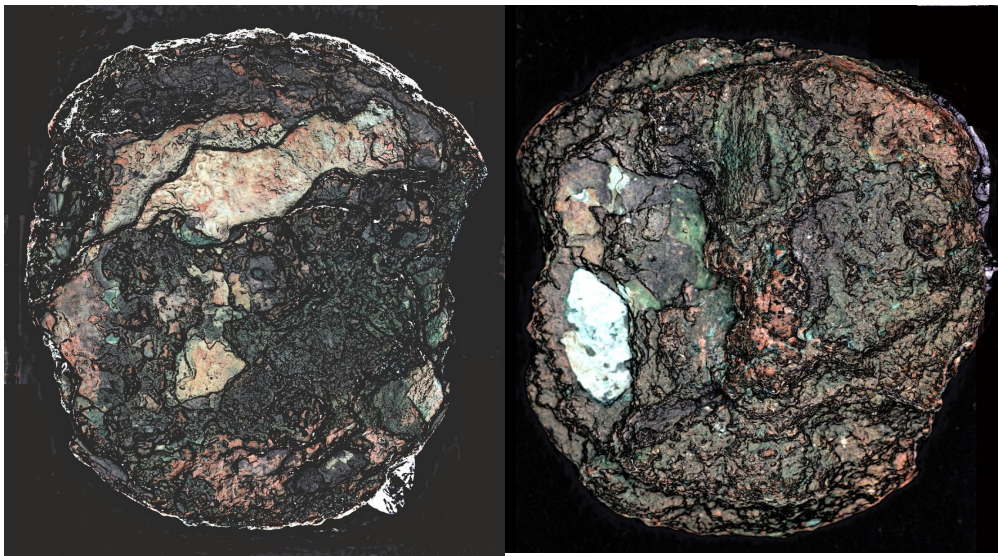
Fig. 31 Both sides of Fragment D in 2005. ©2005 Antikythera Mechanism Research Project. All rights reserved.
