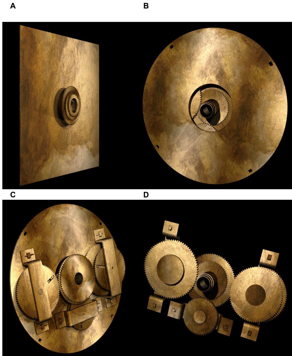
Fig. 37 Computer Reconstructions of the Superior Planet Module. ©2011 Tony Freeth, Images First Ltd. All rights reserved.
