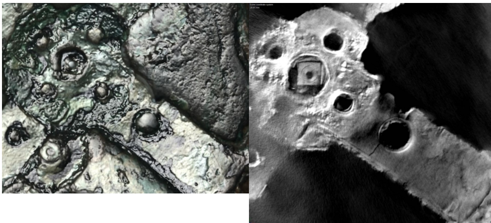
Fig. 13 Apparent bearing in the 4 o'clock position. ©2005 Antikythera Mechanism Research Project. All rights reserved.
