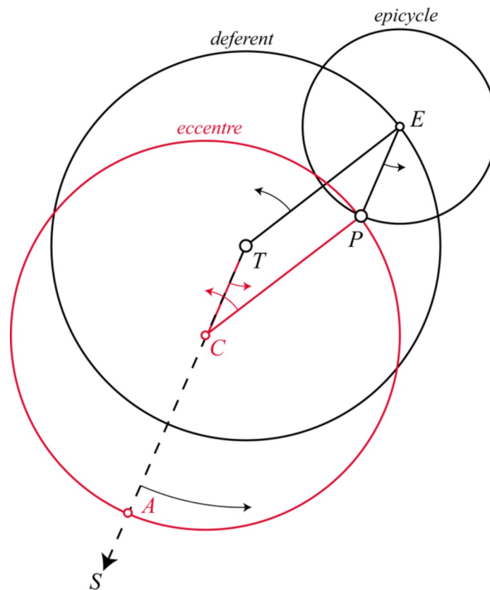
Fig. 26 Deferent and epicycle model (black) and equivalent eccentre model (red) for a superior planet. ©2011 Tony Freeth, Images First Ltd. All rights reserved.
