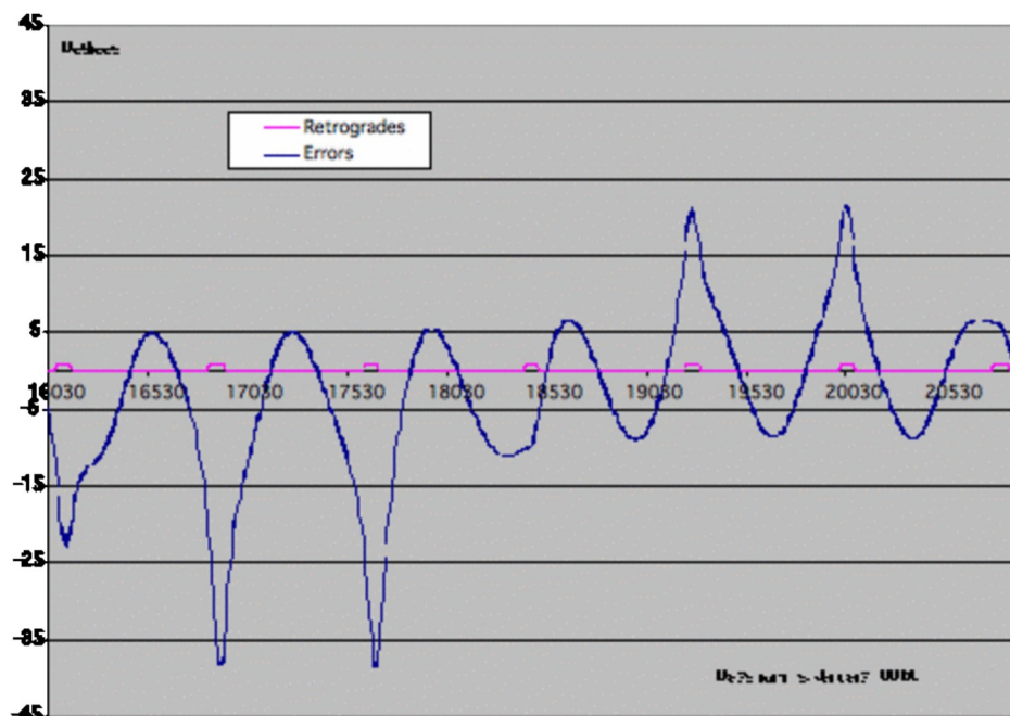
Fig. 39 Errors in deferent and epicycle theory for the planet Mars, middle seven retrogrades in 1st century BC.
