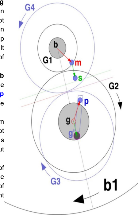
Fig. 41 Geometry of Superior Planetary Mechanisms. ©2011 Tony Freeth, Images First Ltd. All rights reserved.
