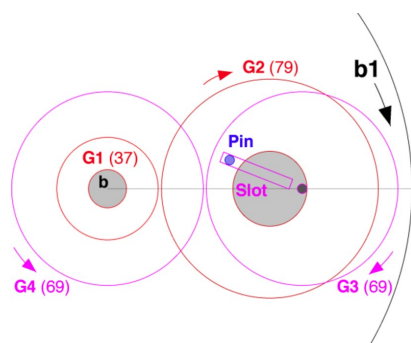
Mars—based on 37 synodic cycles in 79 years.
