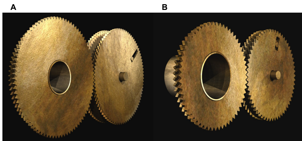
Fig. 36 Computer Reconstructions of Jupiter and Saturn mechanisms. ©2011 Tony Freeth, Images First Ltd. All rights reserved.
